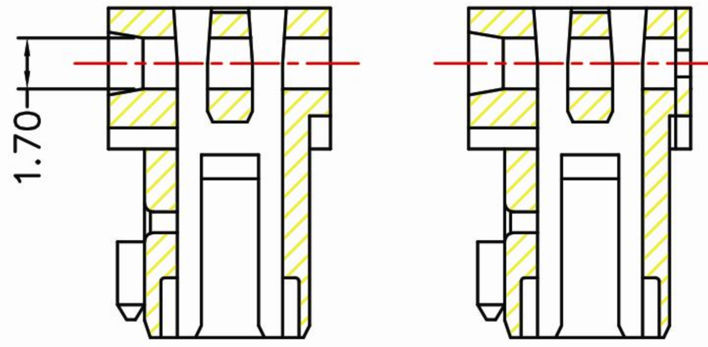
SECTION: B-B
