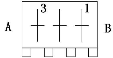
M7235-3-AB-0 (2)
